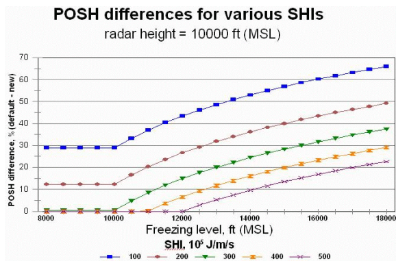
Figure 6. Differences in POSH estimates between the new and default WTSM offset for various SHIs at a radar height of 10000 feet (MSL) and freezing levels of 8000 to 18000 feet (MSL). The curves represent differences in POSH estimates for SHI values for various freezing levels. The POSH estimates using the new WTSM offset will be lower.
