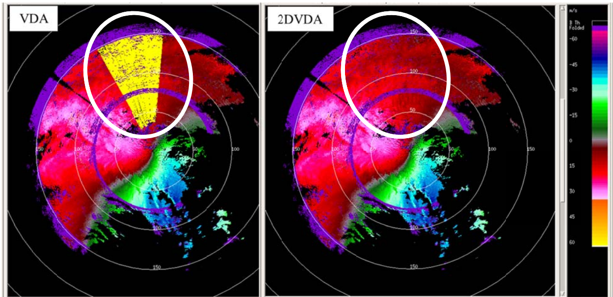
Figure 2. Hurricane Irene August 28, 2012 from Upton, NY WSR-88D (KOKX) at 07:21Z at 0.5 deg elevation. Circulation center is 150 n mi south-southwest of radar. Legacy VDA dealiased \frac{1}{2} deg azimuthal resolution velocity product is on the left, the 2DVDA dealiased product is on the right. Note large yellow wedge of incorrectly dealiased velocities for the legacy VDA (see white ovals). Range rings are every 50 n mi.
