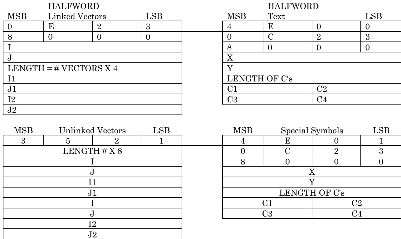
Figure 3-9. Map Message Packet - Packet Codes 0E23, 4E00, 3521 and 4E01 (Sheet 2)
